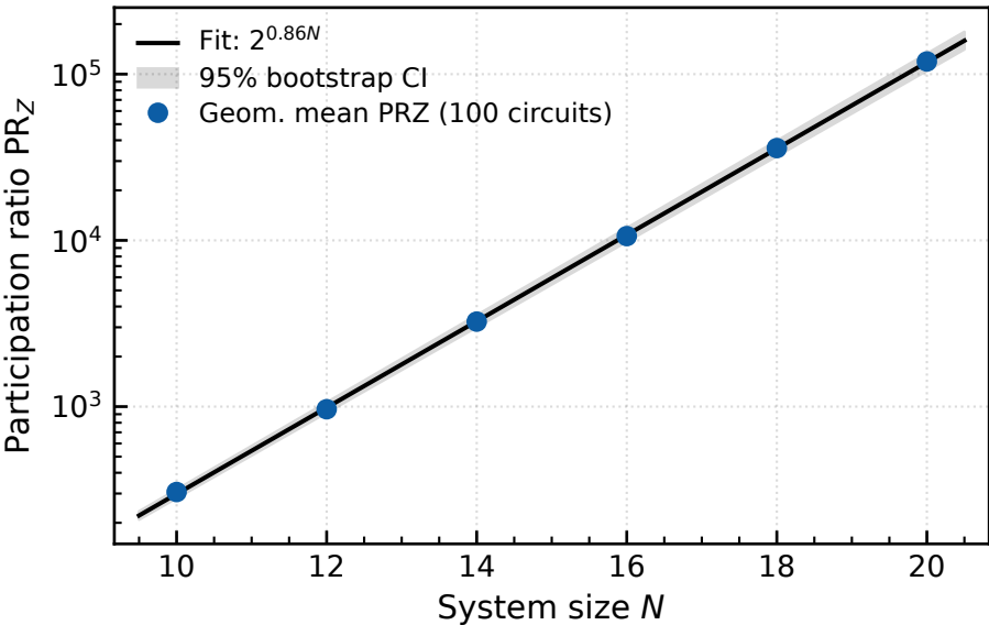
Z-basis PR scaling (brickwork L = 5 )
